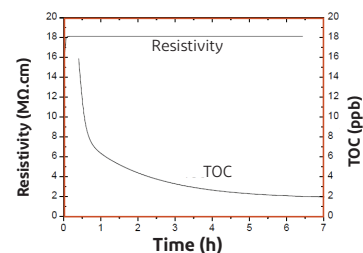
Figure 2: Resistivity and TOC Rinse Performance
